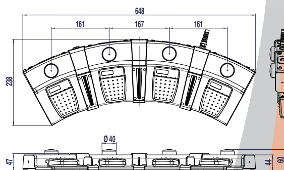
Modular base
