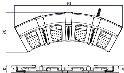
Modular base
