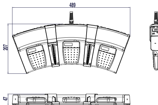
Modular base
